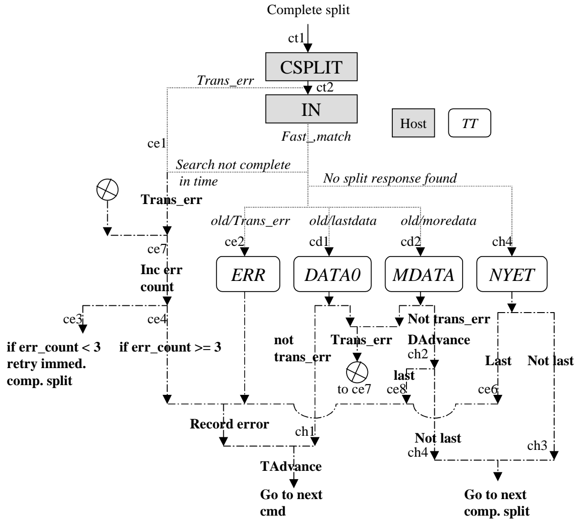
Figure 11-85. Isochronous IN Complete-split Transaction Sequence
