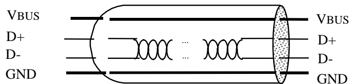
Figure 4-2. USB Cable
